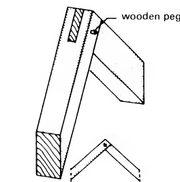
13 Simple tenon joint connecting two rafters
